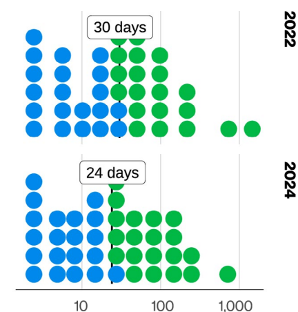
Figure 42. Distribution of dwell time in days in non-Actor-disclosed breaches per year (n for 2022=93 – 2.32 breaches/dot) (n for 2024=248 – 6.20 breaches/dot)
